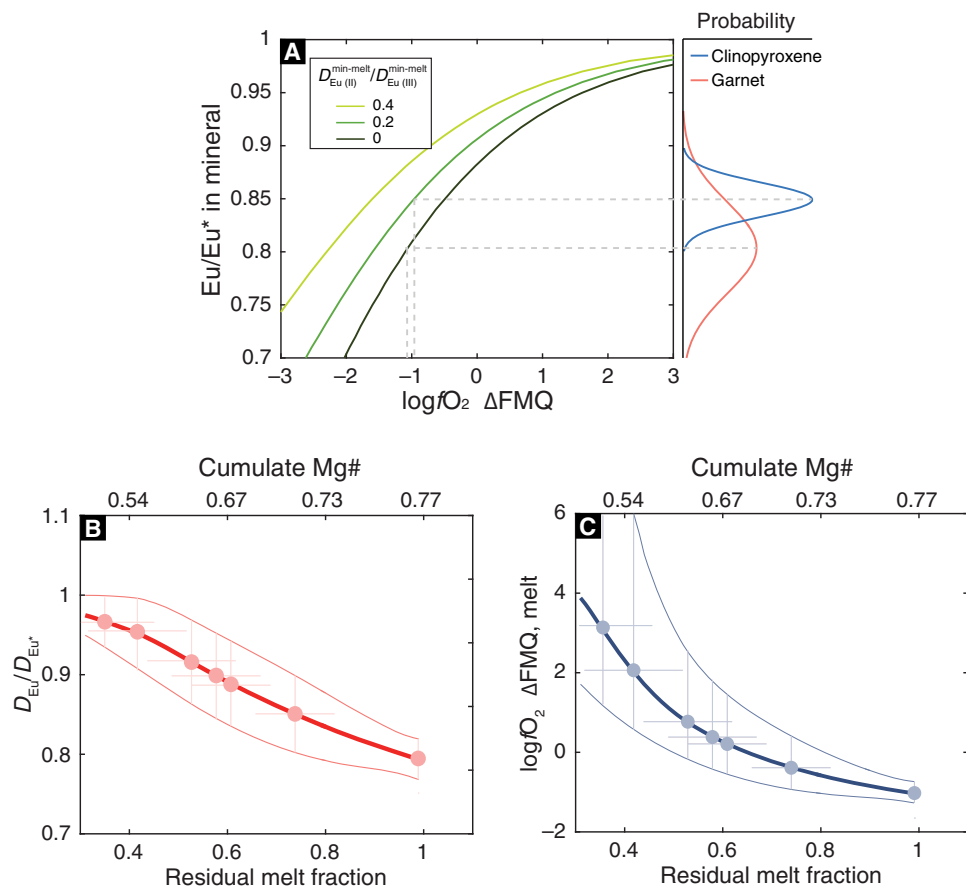
Fig. 2. Magma redox conditions calculated from garnet and clinopyroxene Eu anomalies. (A) Estimating fO_2 of primitive magma. Garnet and clinopyroxene Eu/Eu^* plotted on the contours of D_{Eu(II)}^{min-melt}/D_{Eu(III)}^{min-melt} . The probability distribution is for sample CC-ME1, the second most primitive garnet-bearing pyroxenite in this work. (B) Evolution of the bulk Eu partition coefficient relative to D_{Eu^*} (bulk partition coefficient of Eu^{3+} ) during crystal fractionation, calculated using the observed Eu/Eu^* of garnets and an incremental crystal fractionation model (see the Supplementary Materials and Methods). Dots with error bars (95% confidence interval) represent D_{Eu}/D_{Eu^*} values estimated from Eu/Eu^* of garnets in cumulates. Residual melt fraction estimated by converting whole-rock cumulate Mg# to the Mg# of a melt in equilibrium with the cumulate and inferring melt fraction from empirical relationships between melt Mg# and indices of melt fraction, such as K_2O (see the Supplementary Materials and Methods). The uncertainties are from the measured garnet Eu/Eu^* and cumulate-melt Mg# coupling and are propagated into the calculated D_{Eu}/D_{Eu^*} and fO_2 by a Monte Carlo resampling method (see the Supplementary Materials and Methods). Thick red line demarcates median values, and thin red line displays 95% confidence interval envelope. The total Eu partition coefficients in (B) were converted to fO_2 in (C). Clinopyroxenes show the same Eu/Eu^* -Mg# trend as garnet (Fig. 1), but we use garnet data to calculate the redox paths because the perfect incompatibility of Eu^{2+} in garnet simplifies Eq. 1 and reduces uncertainty.
